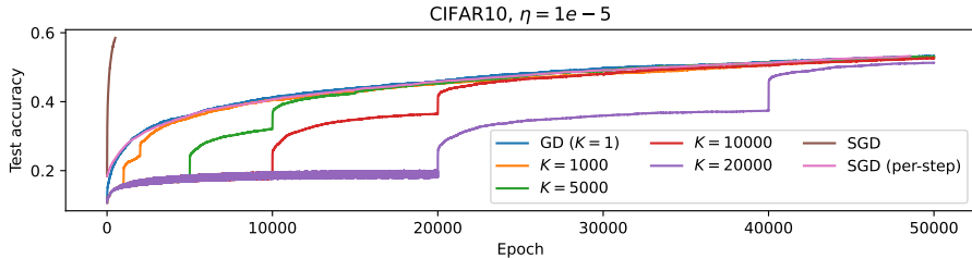
Figure 2: Iterative linearisation on CIFAR10 with large K
